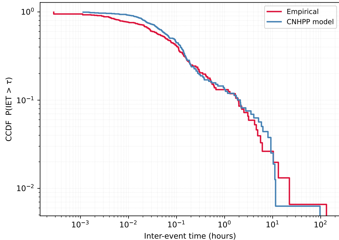
User 1354320169 - Empirical vs CNHPP model
